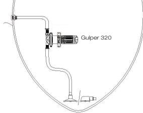
Typical installation as a Remote Mounting bilge pump
